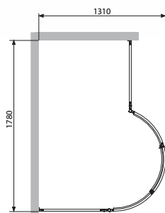
Parant Center + 2 x wand 70 + 2 x SP koppelstrip.
